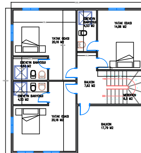
1. KAT PLANI 110 M 2
