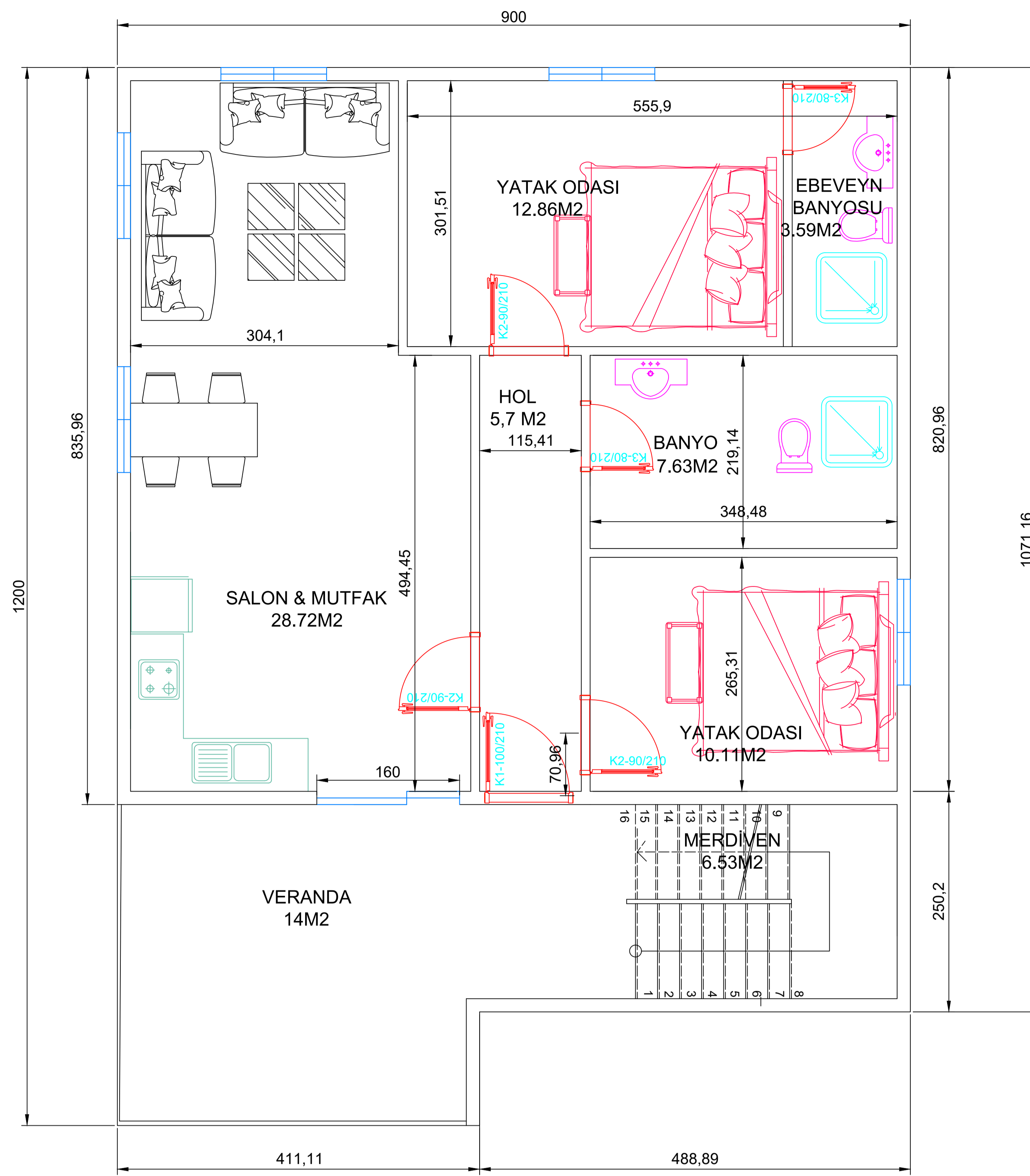
ZEMİN KAT PLAN 98M 2
