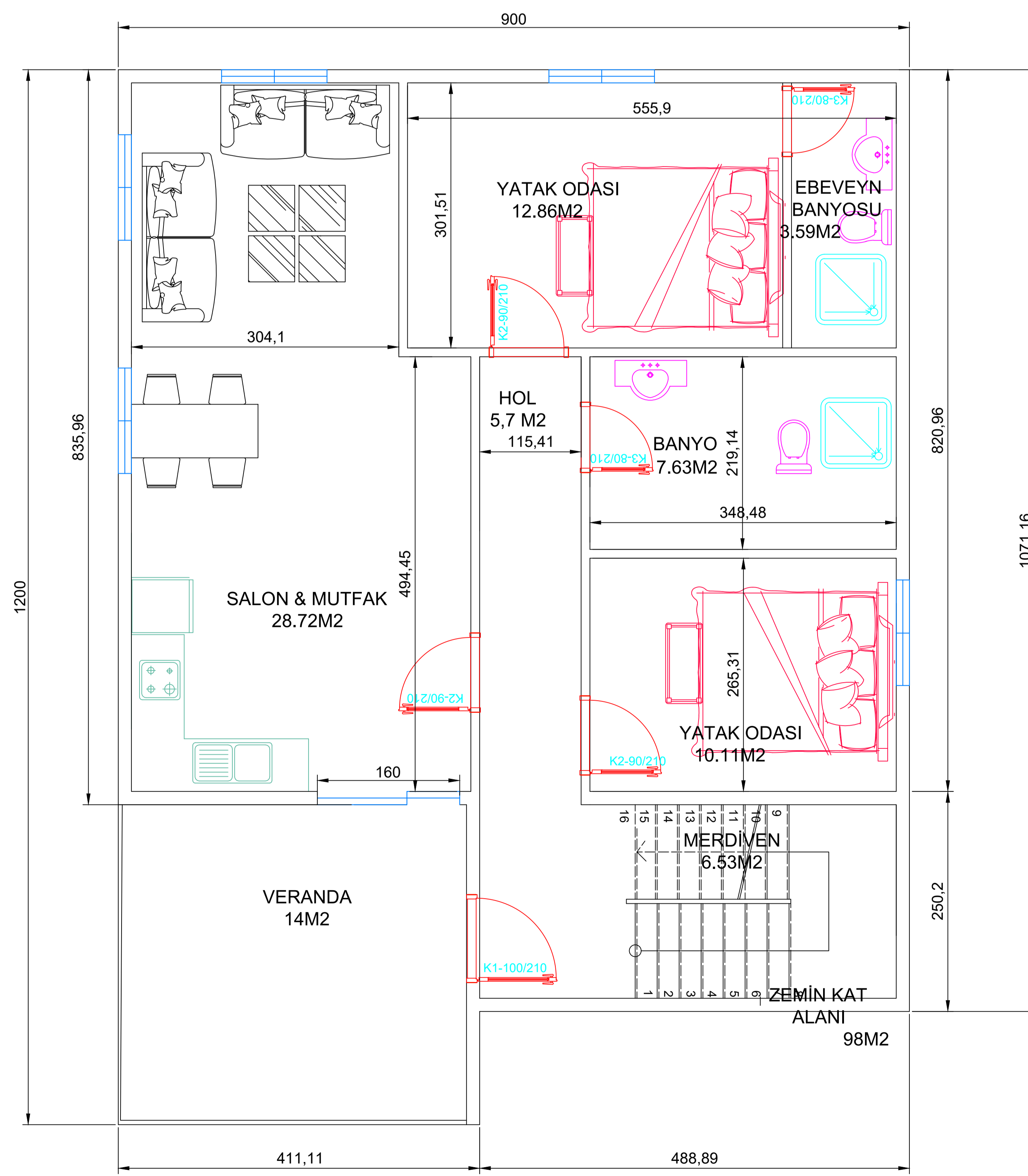
1.KAT PLAN 98M 2
