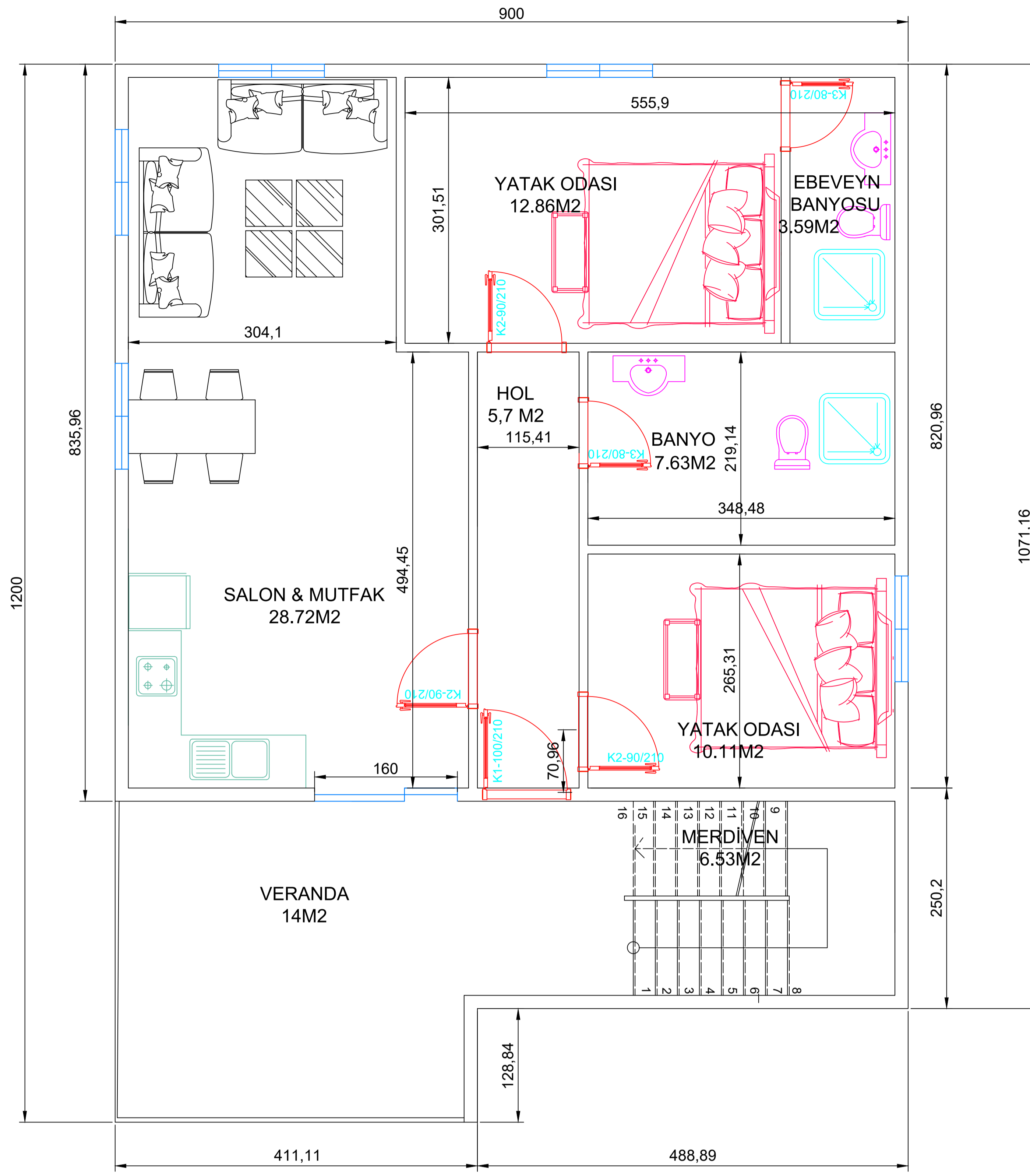
ZEMİN KAT PLAN 101M 2
